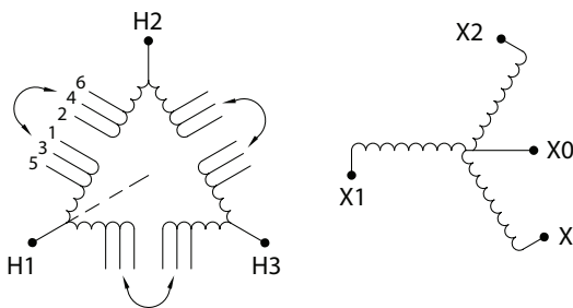
WD4 wiring diagram
