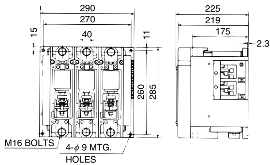
SH-V600(Mass:22kg)
