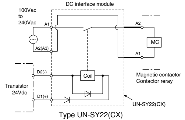
(2) Relay Output
