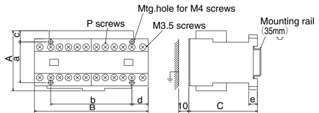
Fig.2 SD-QR type
