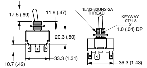
17 Amp, 4 Pole
