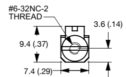
Screw Terminal
