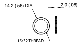
Knurled Nut
