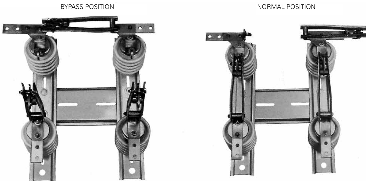
Figure 4. D73-3P 600 A 3-pull oil circuit recloser bypass switch.
