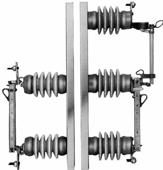
Figure 5. Fused disconnect and companion switch combination.
