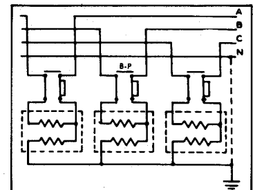
3 single-phase regulators three-phase-wye-3 or 4 wire
