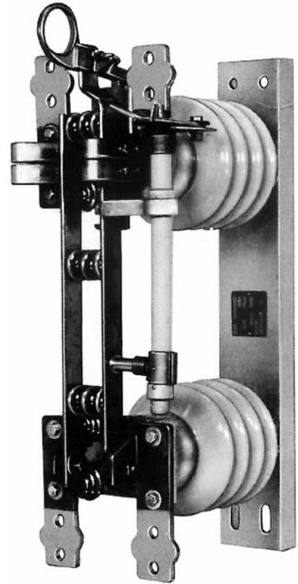
Figure 7. HB-65 station-class, 600 A voltage regulator bypass switch.
