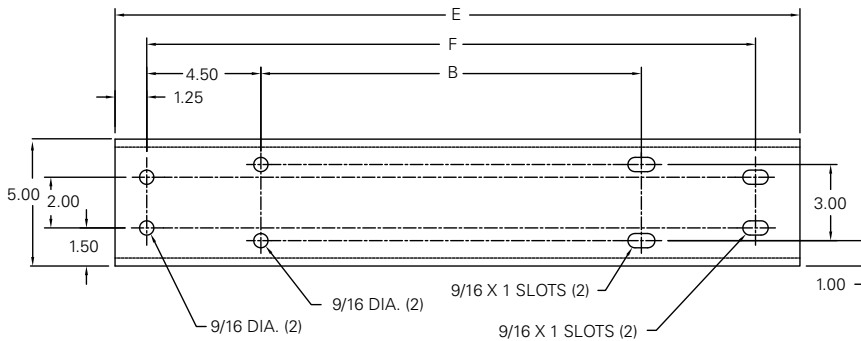
P-72 base dimensions
