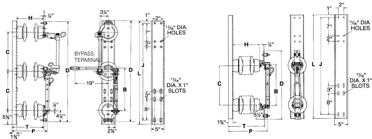
Figure 6. Fused disconnect switch (left) and companion switch (right).
