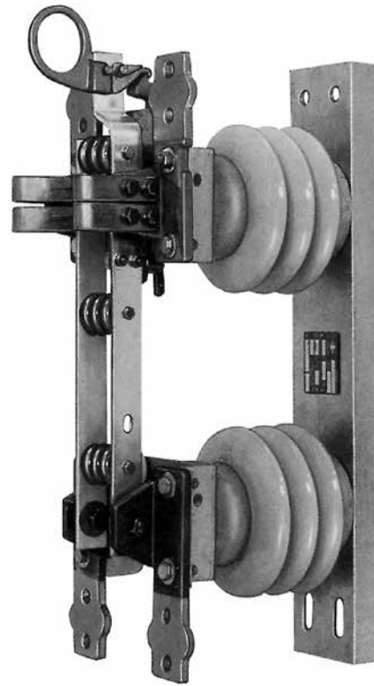
Figure 8. HB-65, 600 A current transformer bypass switch.
