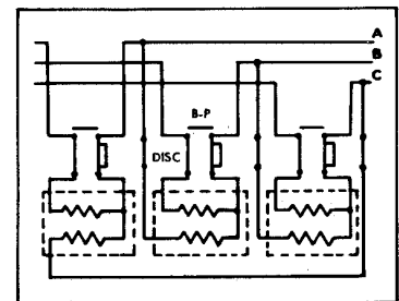
3 single-phase regulators three-phase-delta-3 wire
